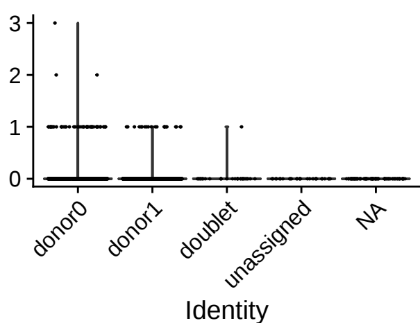
DPB1.677.01
