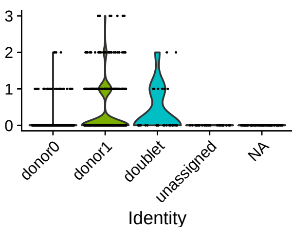
DPB1
