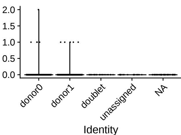
DPB1.50.01
