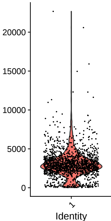
nCount_RNA
