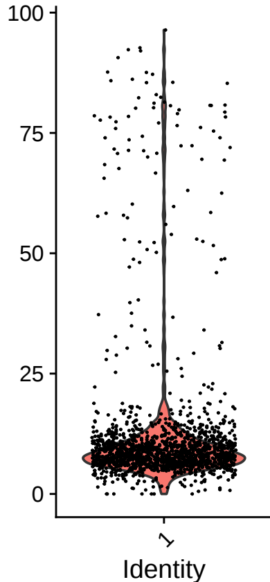
percent.mt
