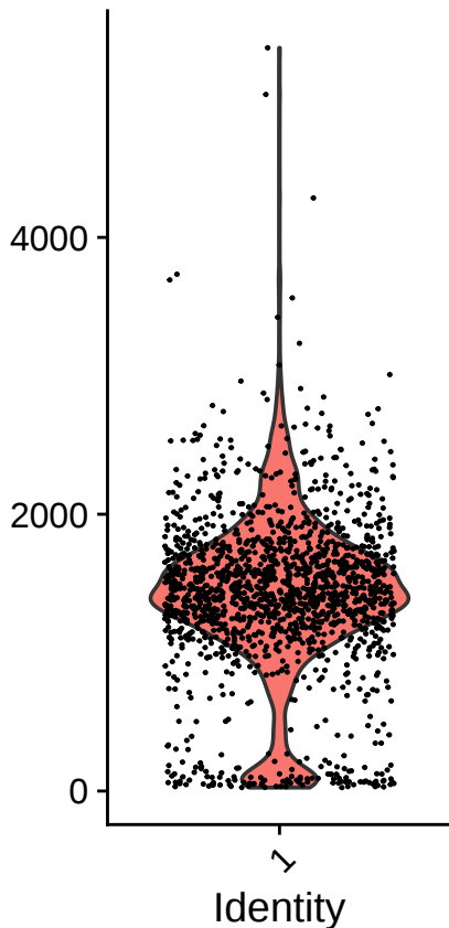
nFeature_RNA
