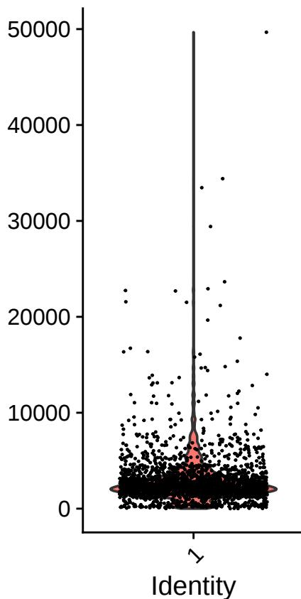
nCount_RNA
