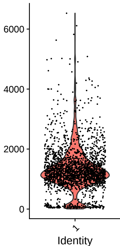
nFeature_RNA
