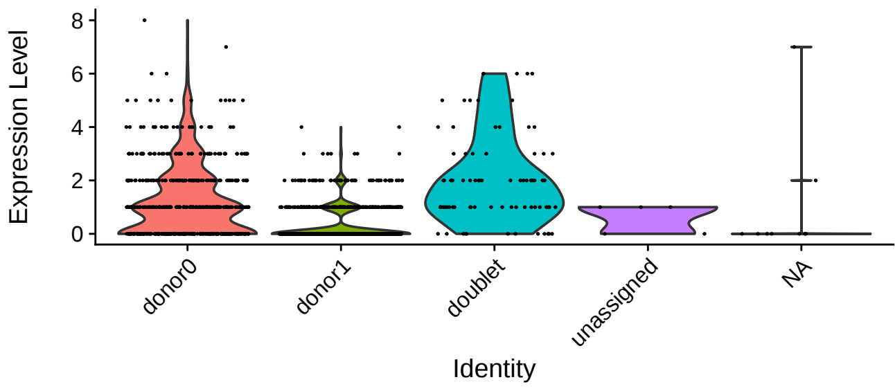
DRB1-11:03:01-PASC-Sample-D
