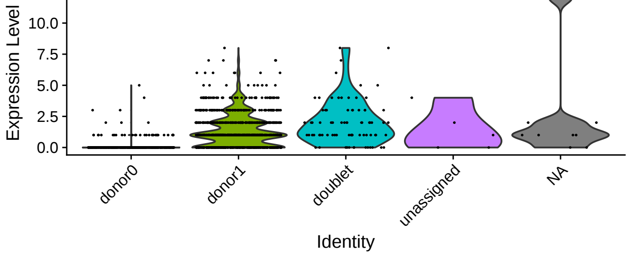
B44:03:01:01-Healthy-Sample-D
