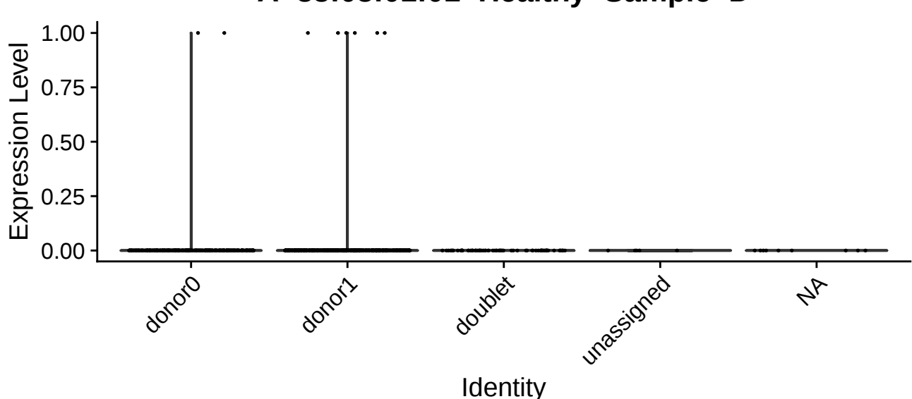
C-07:06:01:01-Healthy-Sample-C-and-Healthy-Sample-D
