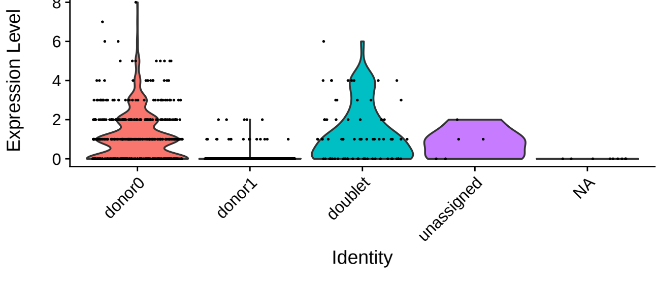
B44:03:01:01-Healthy-Sample-D
