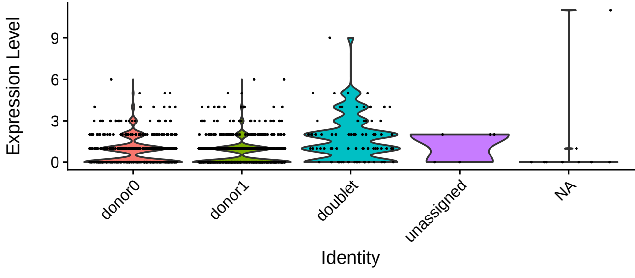
A01:01:01:01-Healthy-Sample-D
