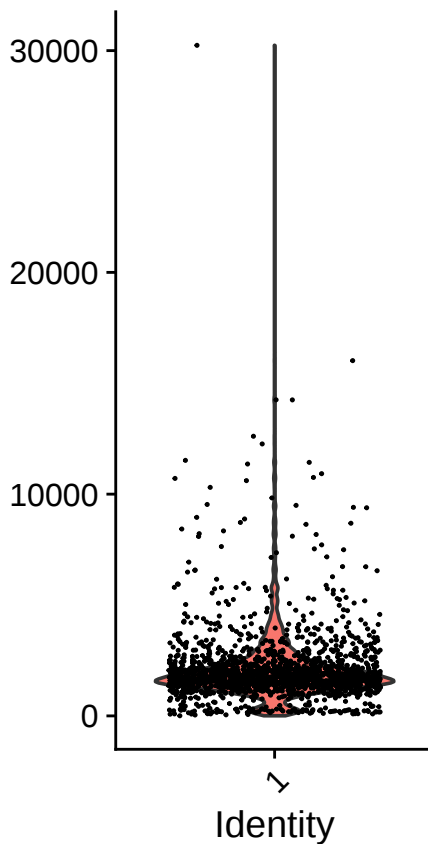
nCount_RNA
