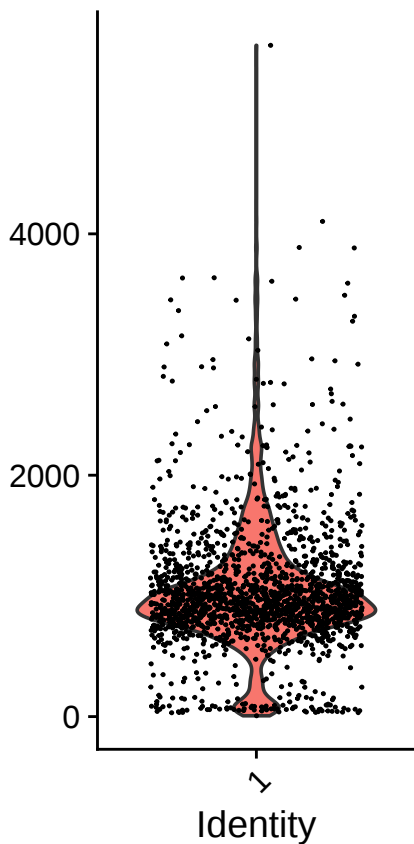
nFeature_RNA
