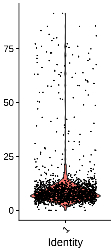
percent.mt
